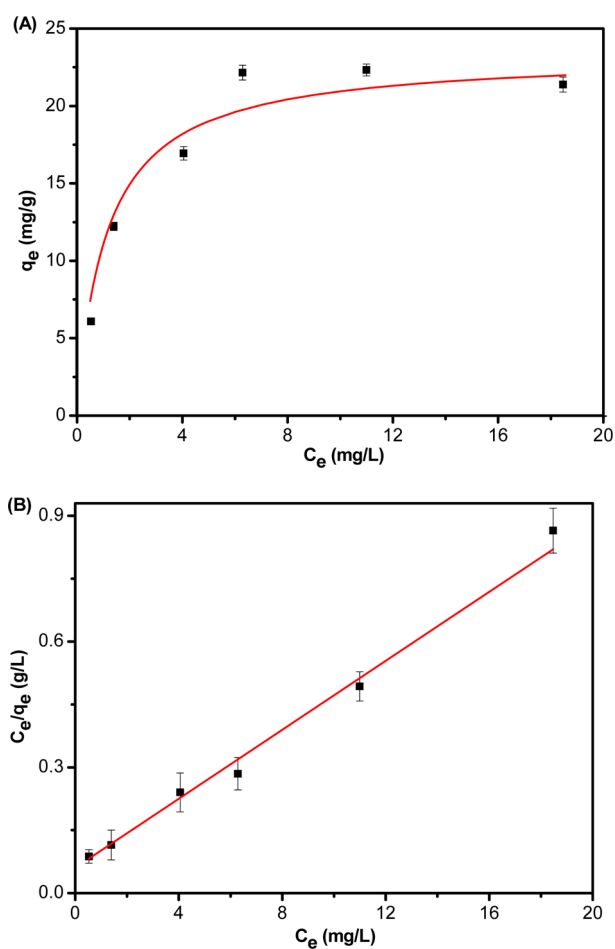
Figure 6. (A) Adsorption isotherms and (B) corresponding Langmuir plots of Congo red on SiO 2 @ \gamma -ALOOH (Boehmite) core/sheath fiber membranes for over 90 min.
