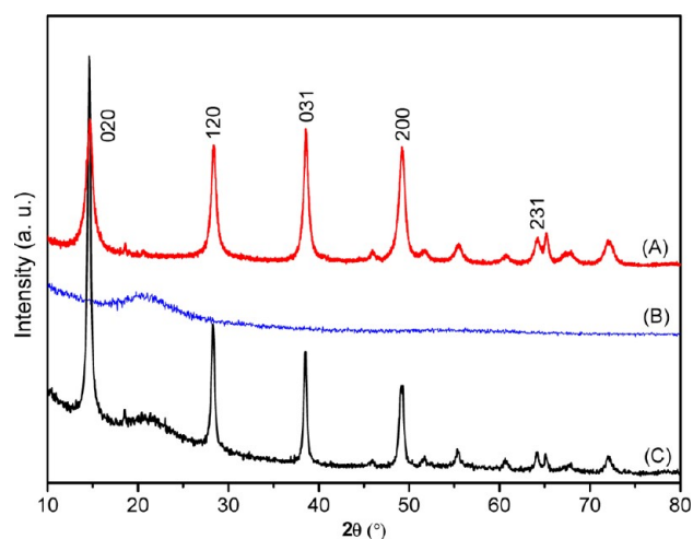
Figure 2. XRD patterns of (A) Boehmite particles, (B) SiO 2 fibers, and (C) SiO 2 @ \gamma -AlOOH (Boehmite) core/sheath fibers.
