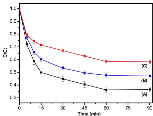
Figure 9. Adsorption rates of Congo red on a \text{SiO}_2@ \gamma\text{-ALOOH} (Boehmite) core/sheath fiber membrane after the (A) first, (B) second, and (C) third cycles.
