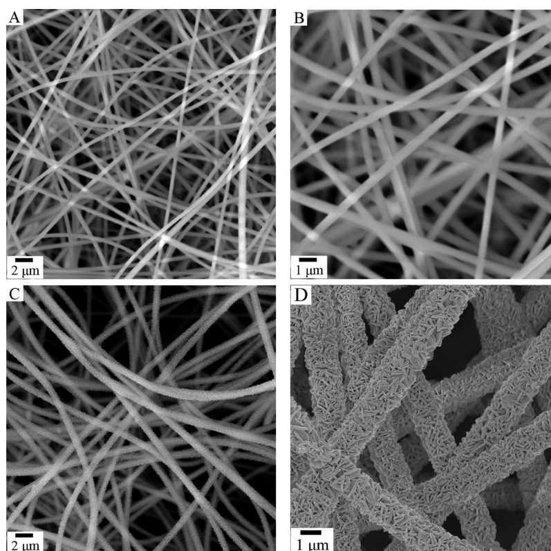
Figure 3. Low- and high-magnification SEM images of (A and B) SiO 2 fibers and (C and D) SiO 2 @ \gamma -AlOOH (Boehmite) core/sheath fibers.
