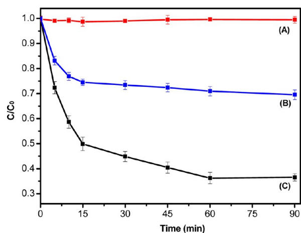
Figure 5. Adsorption rates of Congo red on (A) SiO 2 fiber membrane, (B) Boehmite powder, and (C) SiO 2 @ \gamma -ALOOH (Boehmite) core/sheath fiber membrane, respectively.
