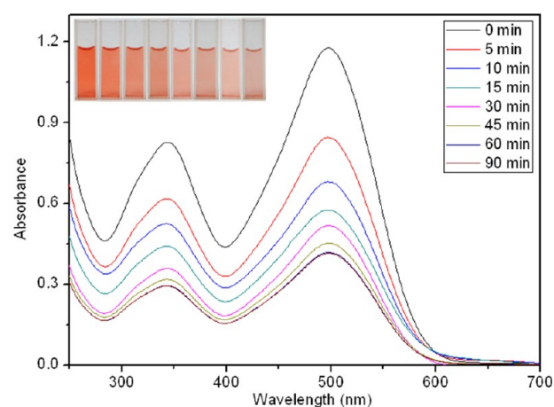
Figure 4. Absorption spectra of Congo red in the presence of a SiO 2 @ \gamma -AlOOH (Boehmite) core/sheath fiber membrane after time intervals of 0, 5, 10, 15, 30, 45, 60, and 90 min. The insets are the corresponding digital photographs of Congo red solutions at the same time when the UV–vis spectra are taken.
